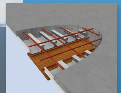
Slab Beam
