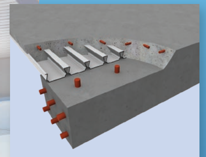
Precast Beam
