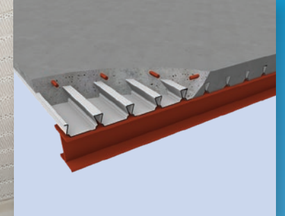
Steel Beam
