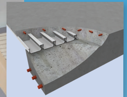
Reinforced Concrete Beam
